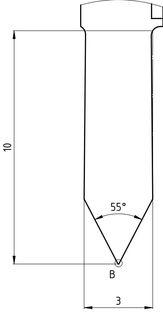
A (10 : 1)
